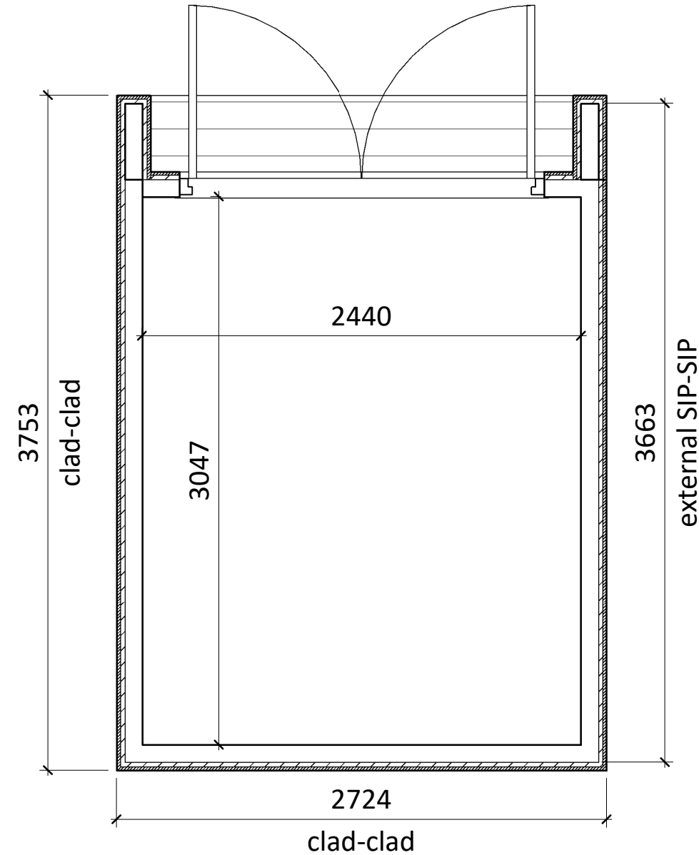
1 01 General Floor Plan 1 : 30
