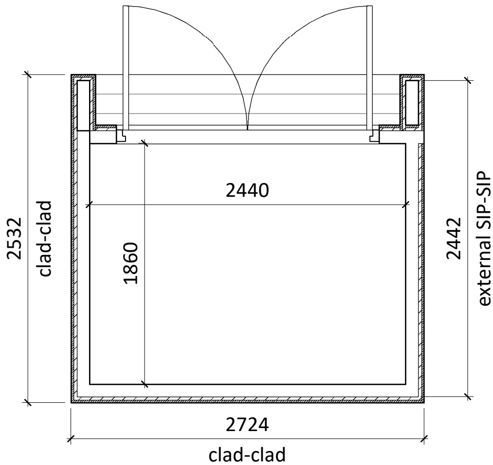
1 01 General Floor Plan 1 : 30
