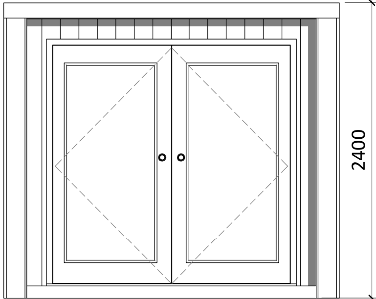
3 Front Elevation 1 : 30
