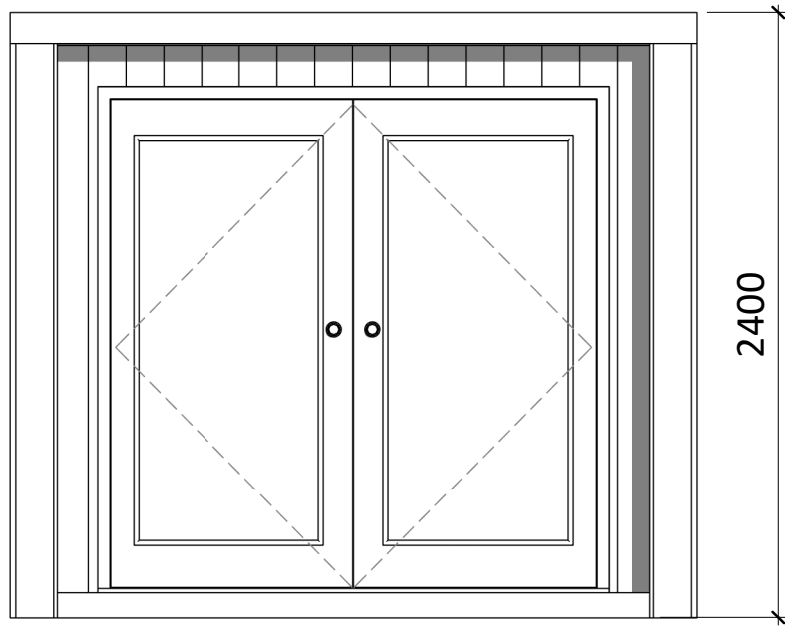
3 Front Elevation 1 : 30
