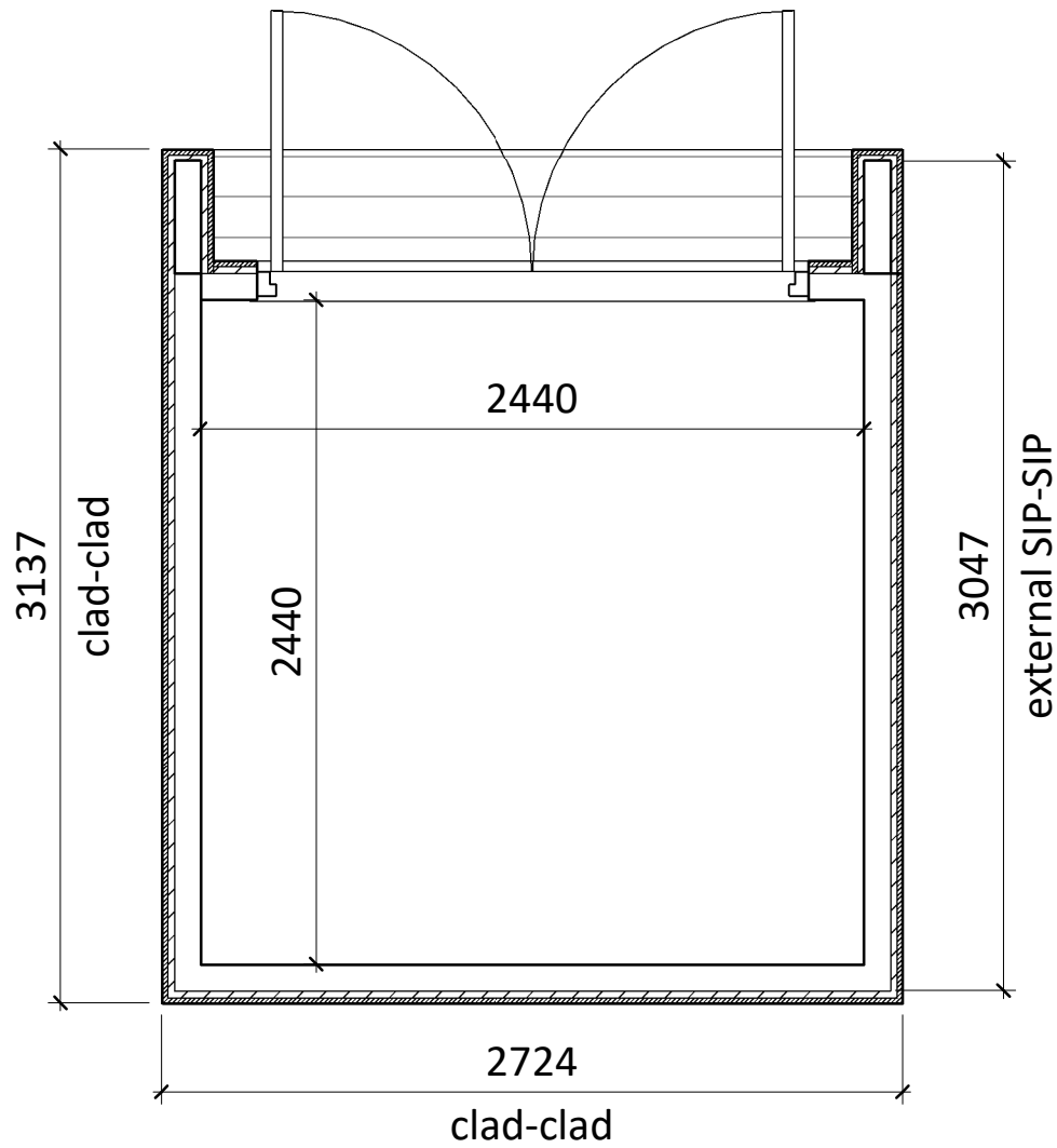
1 01 General Floor Plan 1 : 30
